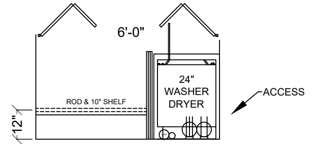
75" CLOSET W W/D PREP & W/D
