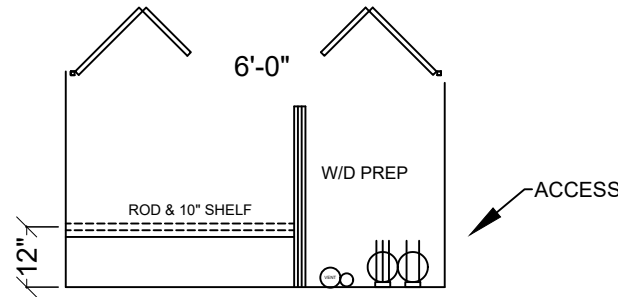
75" CLOSET W W/D PREP IN CLOSET
